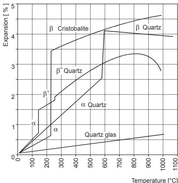
Figure 1. Volumetric changes of different quartz sands depending on temperature
