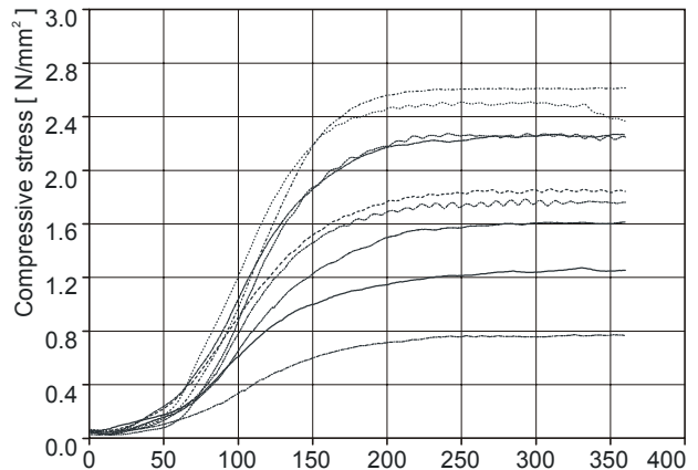
B = Bentonite; W = Water — 4% B.; 2.5% W. — 7% B.; 2.5% W. — 10% B.; 2.5% W. ..... 4% B.; 4.0% W. — 7% B.; 4.0% W. — 10% B.; 4.0% W. ..... 4% B.; 6.0% W. — 7% B.; 6.0% W. — 10% B.; 6.0% W.
