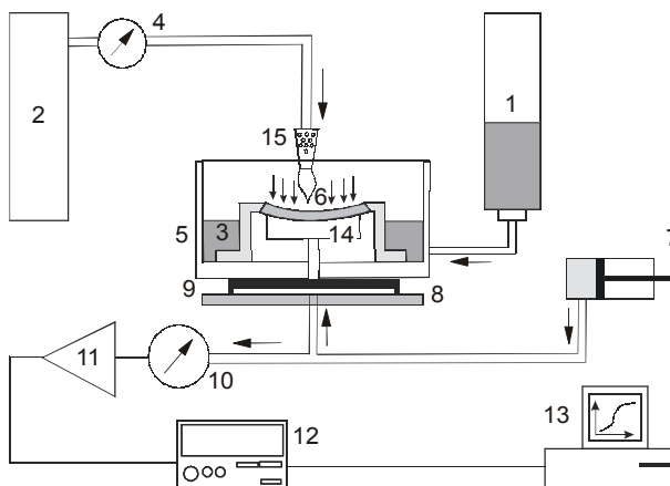
Figure 2. The modified device for measuring compressive stresses. Components: 1 - vessel with cooling water, 2 - acetylene tank, 3 - sample holder, 4 - manometer, 5 - gauge housing, 6 - test sample, 7 - compressor, 8 - base plate, 9 - counter-plate, 10 - pressure sensor, 11 - amplifier, 12 - measuring switch (A/D converter), 13 - computer, 14 - measuring probe, 15 - burner
