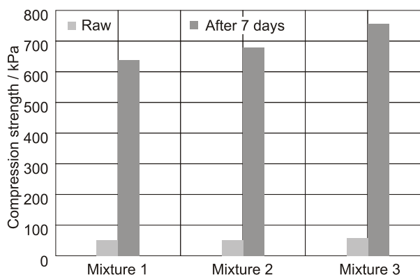
Figure 5. Compression strength values of testing cylinders from LF slag
