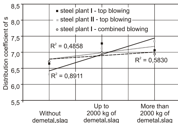
Figure 2. Effect of demetallized slag recycling on desulphuration process in oxygen converter Slika 2. Učinak recikliranja demetalizirane troske na proces otsumporavanja u kisikovom konvertoru
