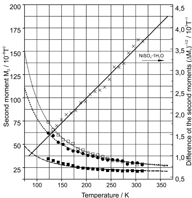
Figure 1. The temperature dependences of NMR second moment M_2 and [\Delta M_2]^{-1/2} for MnSO_4 \cdot 1H_2O (●, ■) and NiSO_4 \cdot 1H_2O (□, ×) measured at B_{r_1} = 0,331 T (●, ■) and B_{r_2} = 0,705 T (□, ×). Slika 1. Ovisnost temperature o drugom momentu MRJ i [\Delta M_2]^{-1/2} za MnSO_4 \cdot 1H_2O (●, ■) i NiSO_4 \cdot 1H_2O (□, ×) izmjeren pri B_{r_1} = 0,331 T (●, ■) i B_{r_2} = 0,705 T (□, ×).
