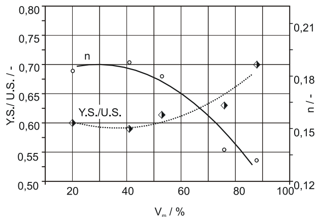
Figure 3. Variation of strain hardening exponent ( n ) and ratio R_{p0.2} / R_m as a function of volume fraction of martensite for DP Steels
