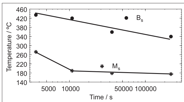
Figure 7. Change of the temperature of the bainitic and martensitic phase transitions with increasing time of 6Mn16 steel pre-soaking at 625°C
