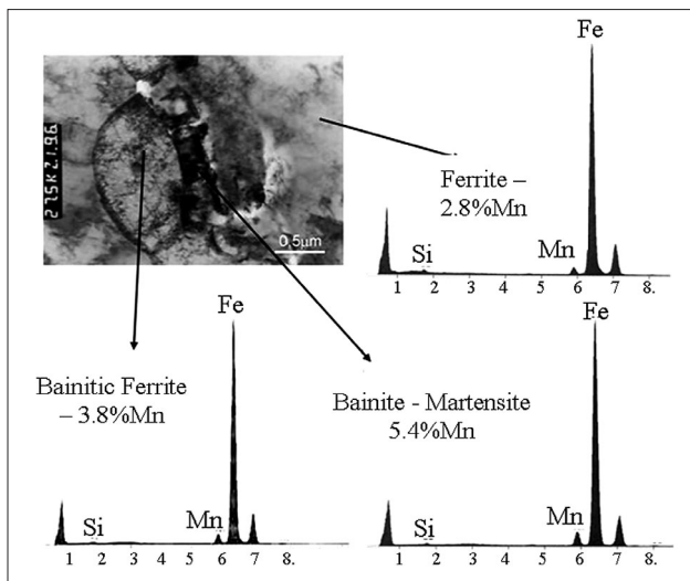
Figure 8. A multi-phase structure with the spectra of characteristic radiation and concentration of alloying elements occurring in the structural components of steel 6Mn16 heat treated from the interval ( \alpha + \gamma ) 700°C/1800s and cooled down at V \approx 12^\circ\text{C/s}
