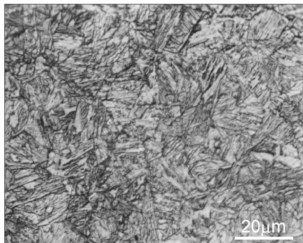
Figure 2. Martensite-bainite structure of 6Mn16 steel after cooling rate 17°C/s.
