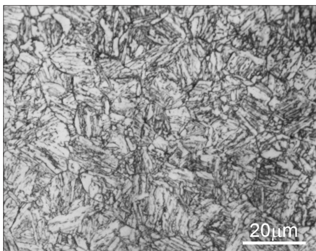
Figure 3. Martensite-bainite structure of 6Mn16 steel after cooling rate 6.82°C/s.
