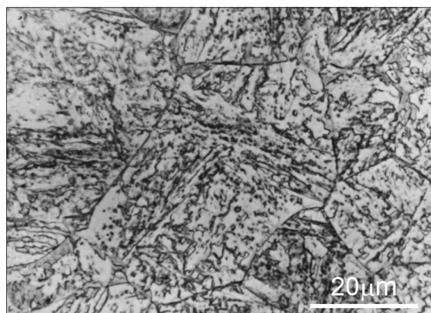
Figure 4. Lower bainite-martensite structure of 6Mn16 steel after cooling rate 0.38°C/s.
