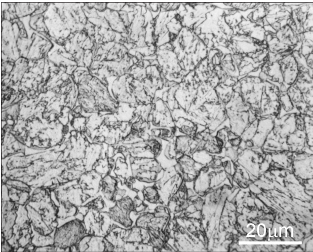
Figure 6. Bainite - polygonal ferrite - martensite structure of 6Mn16 steel after cooling rate 0.008°C/s.
