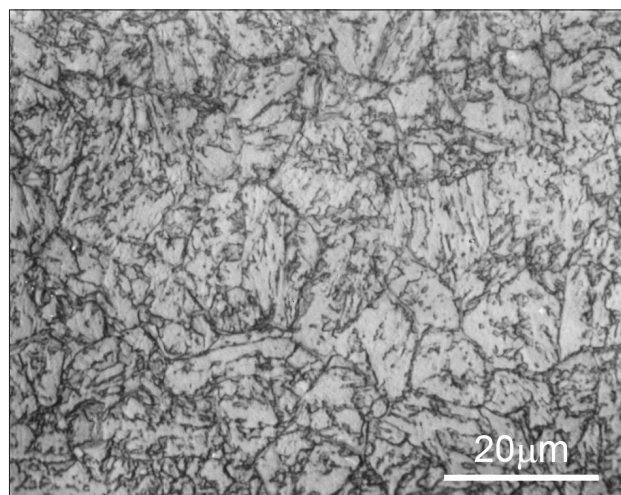
Figure 5. Upper bainite structure of 6Mn16 steel after cooling rate 0.04°C/s.
