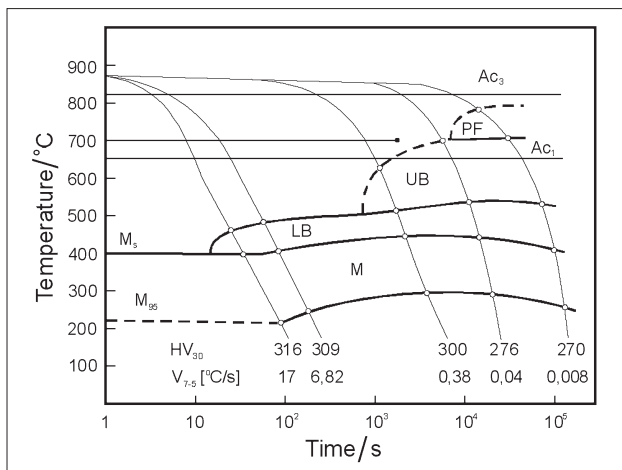
Figure 1. CCT diagram for steel 6Mn16 cooled down from the temperature 875oC/900s.
