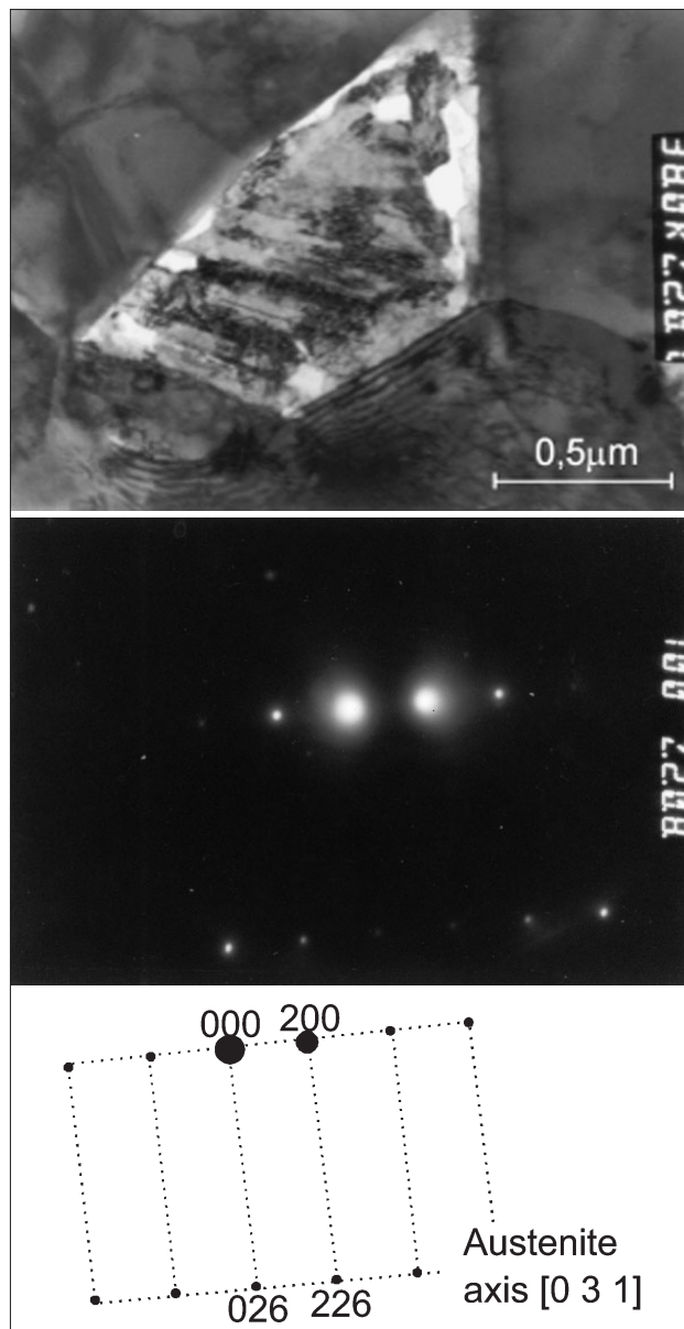
Figure 10. Microstructure of steel 6Mn16 after soaking in the interval ( \alpha + \gamma ) 700°C/1800s and cooled down at V \approx 12^\circ\text{C/s} ; a) bright area, b) diffraction, c) diffraction solution
