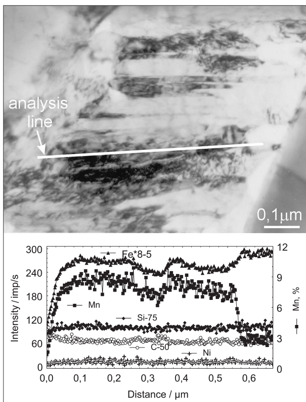
Figure 9. Microstructure of a BM islet in the ferritic matrix of steel 6Mn16 and the concentration of alloying constituents along the line analyzed
